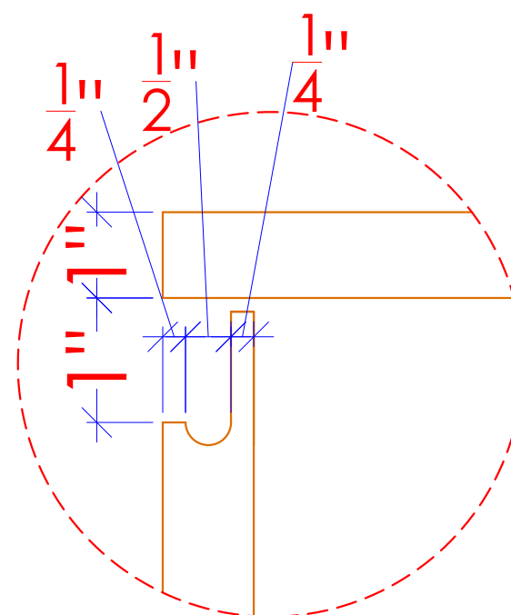
Detail A
